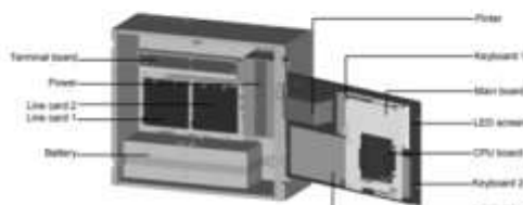
Fig. 1 Internal structure
